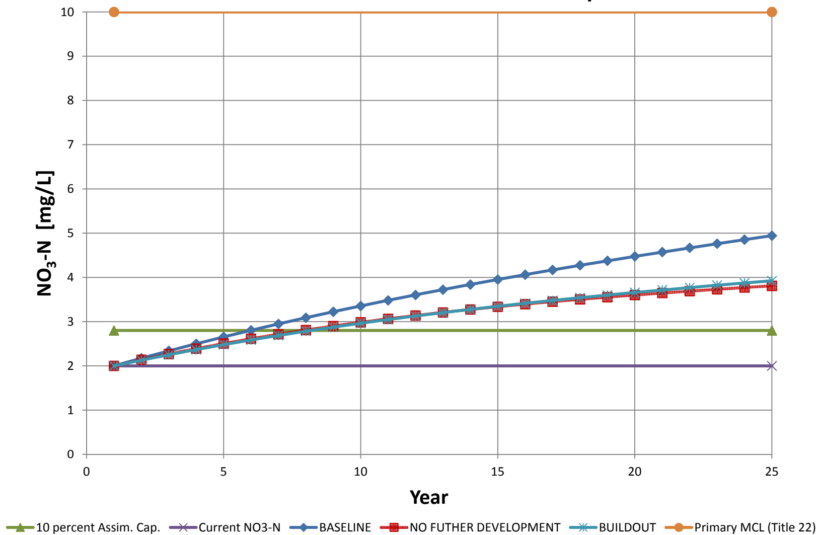
Figure E15 NO 3 -N Concentration Trends Western and Central Area Lower Aquifer
