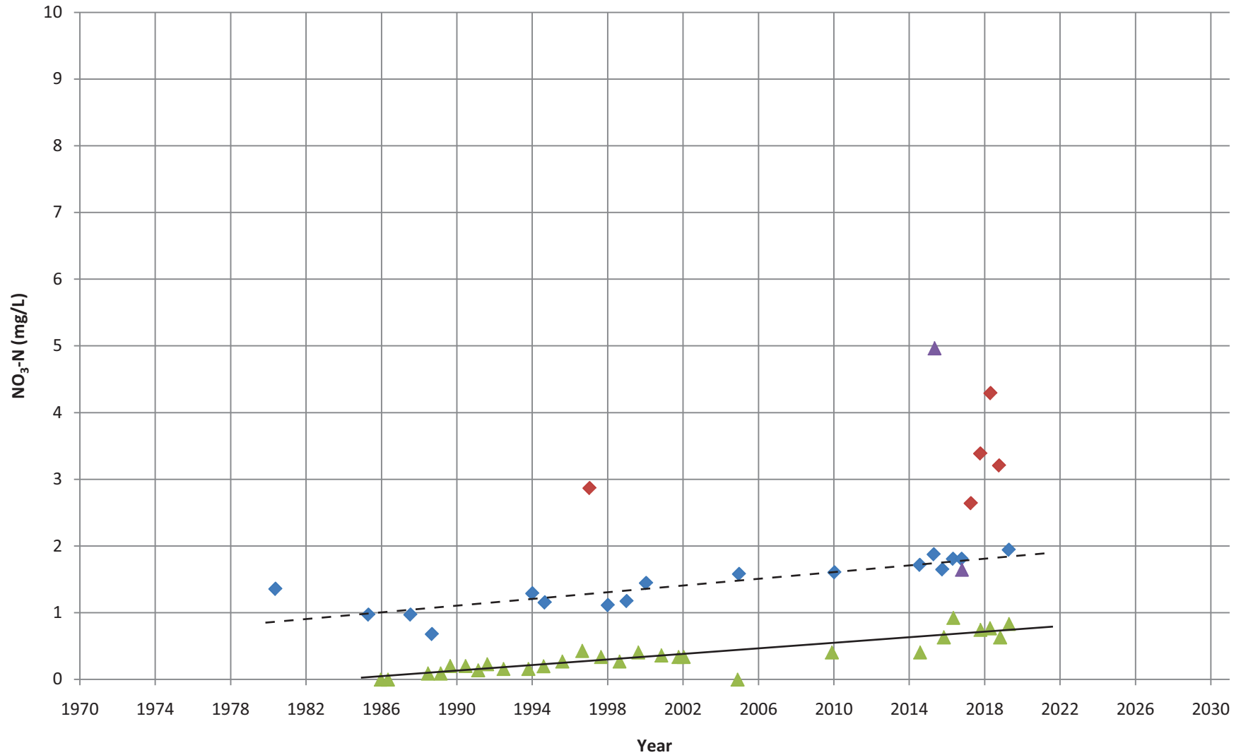
Figure 3 Nitrate-Nitrogen Concentrations LA10 and LA15 2019 Adaptive Management TM
