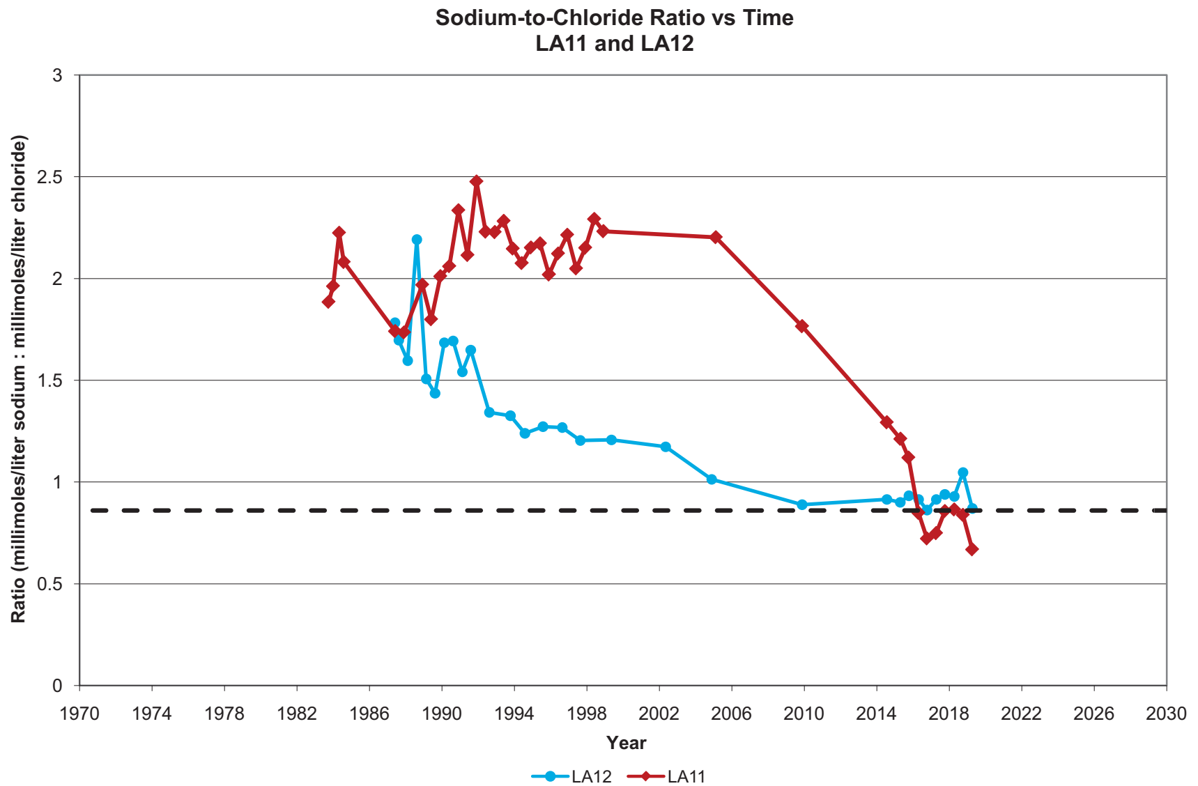
Figure 6 Sodium-to-Chloride Ion Ratios LA11 and LA12 2019 Adaptive Management TM Cleath-Harris Geologists
