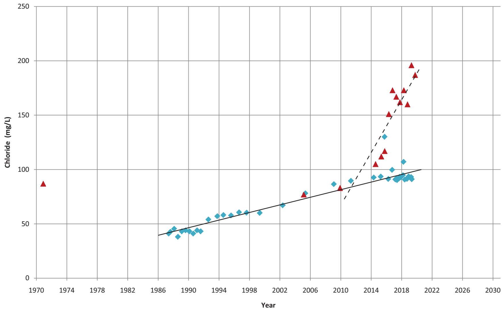
Figure 5 Chloride Conecentrations LA11 and LA12 2019 Adaptive Management TM
