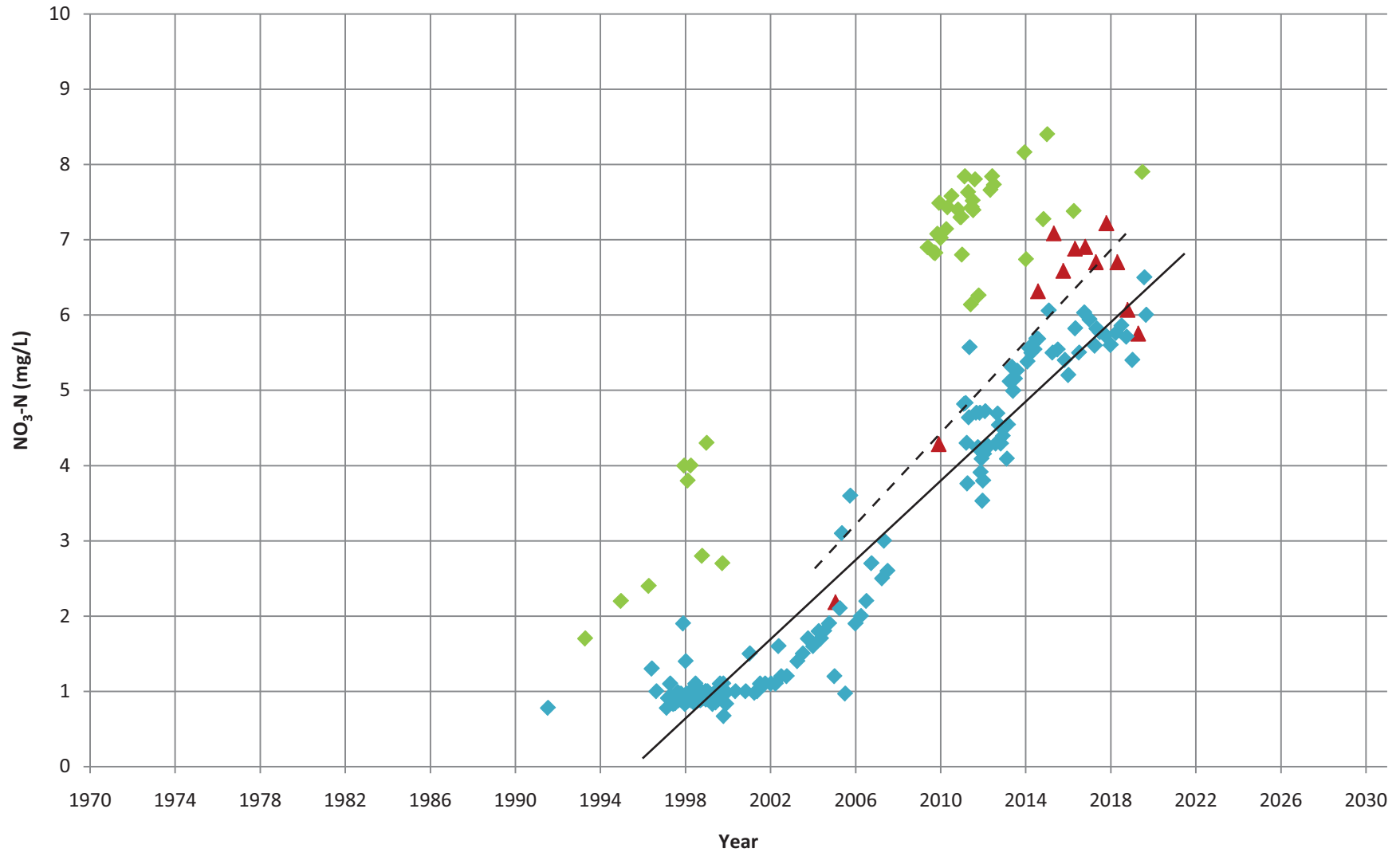
Figure 4 Nitrate-Nitrogen Concentrations LA22 and 17E11 2019 Adaptive Management TM
